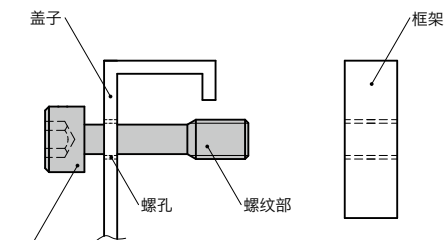
SSC-TF 内六角防脱落螺丝
